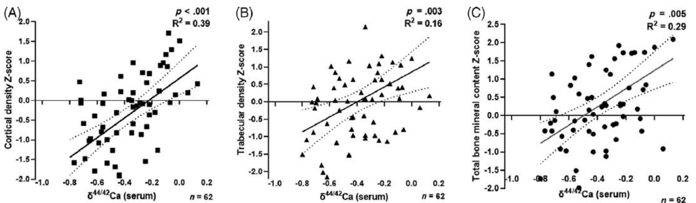
Fig 4. Correlation of \delta^{44/42}\text{Ca}_{\text{serum}} (%) with bone densitometry markers on peripheral quantitative computed tomography scan of the tibia in 62 participants (42 children older than 5 years and 20 adults). Tibial cortical density Z-score (A), trabecular density Z-score (B), and total bone mineral content Z-score (C) showed significant correlations with \delta^{44/42}\text{Ca}_{\text{serum}} , confirming an increase in bone mineral density as bone Ca content increases.
