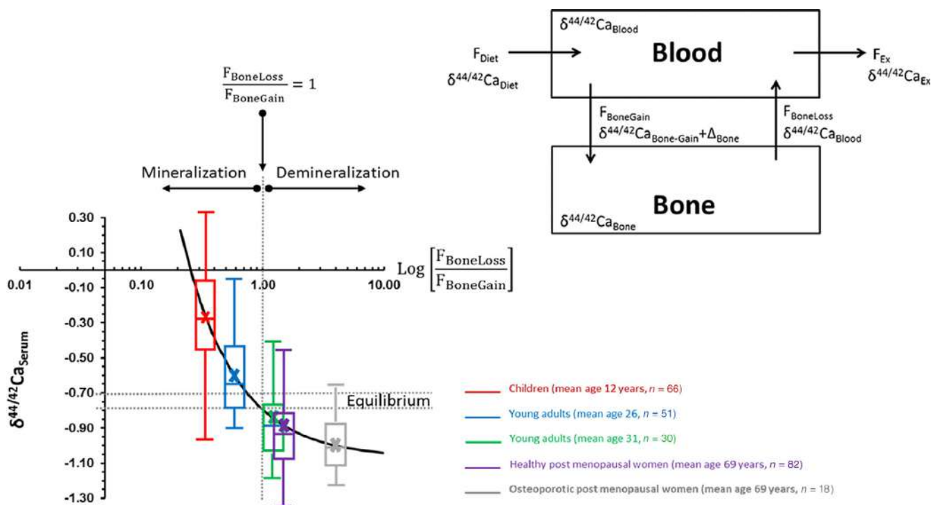
Fig 5. In healthy individuals, the serum Ca isotope composition \delta^{44/42}\text{Ca}_{\text{Blood}} depends on age from childhood (mean age 12 years), young adulthood (mean ages 26 and 31 years in two cohorts), as well as healthy and postmenopausal women (mean ages 69 years for both). Modeling indicates an equilibrium value ( F_{\text{BoneLoss}}/F_{\text{BoneGain}} ratio) between 0.7 and 0.76‰ (gray dotted lines). The more positive values of younger subjects are above the equilibrium value, indicating a positive Ca balance ( F_{\text{BoneLoss}}/F_{\text{BoneGain}} ratio > 1 ) and increasing skeletal mass. In contrast, \delta^{44/42}\text{Ca}_{\text{Blood}} values below the equilibrium values indicate a negative Ca balance ( F_{\text{BoneLoss}}/F_{\text{BoneGain}} ratio < 1 ) and skeletal demineralization with a net loss of bone mass.
